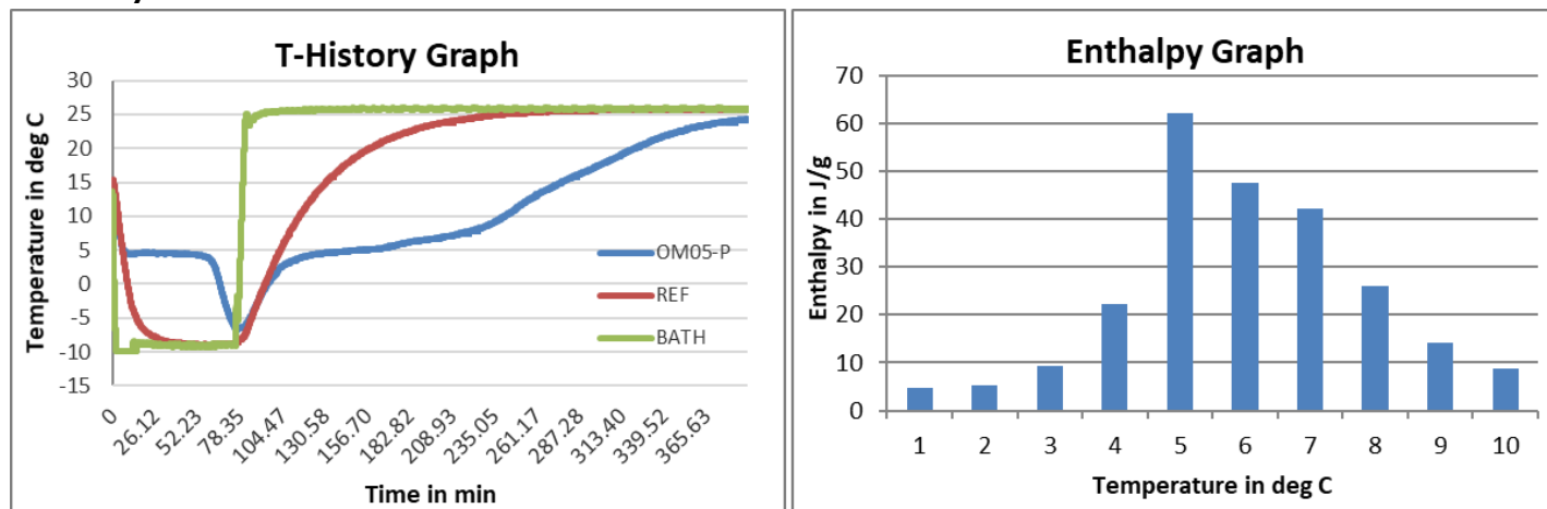
Fig1: T-History Data for OM05-P done in air bath
