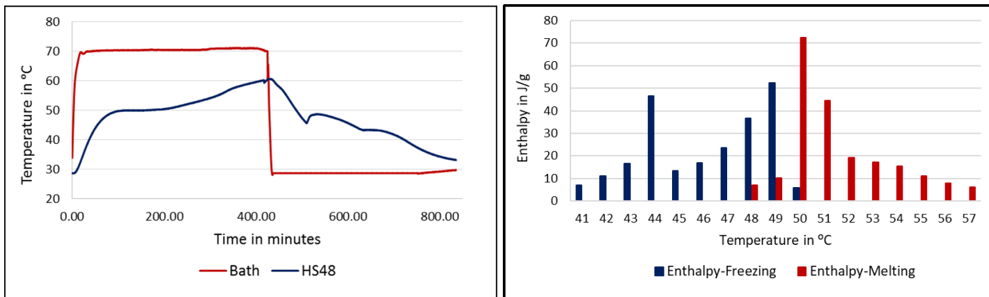
Fig1: T-History Data for HS48 done in air bath
