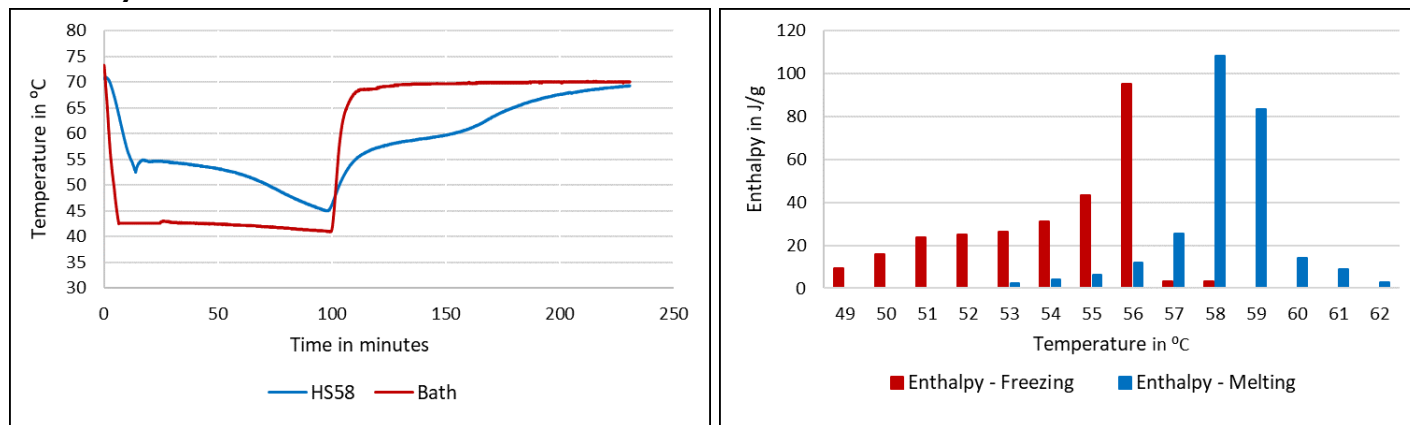
Fig1: T-History Data for HS58 done in air bath
