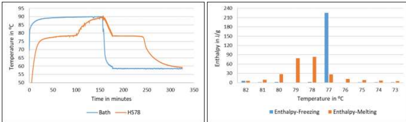
Fig1: T-History Data for HS78 done in air bath
